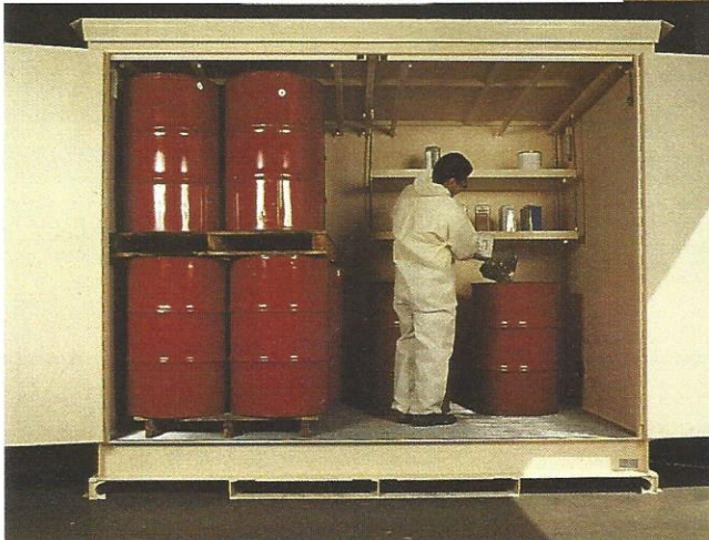
Model #10XR. Two door. For storage and dispensing.
